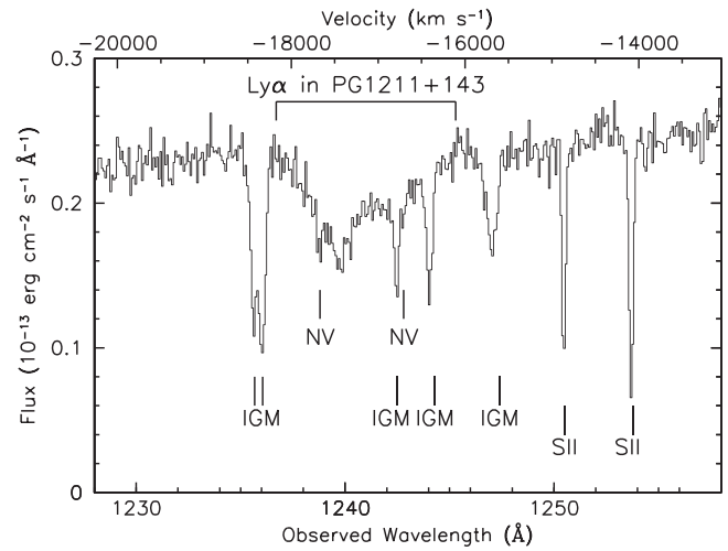
Figure 9. HST -COS G130M spectrum of PG 1211+143 in the wavelength range covering the broad Ly \alpha absorption line profile, the IGM Ly \alpha lines (Penton et al. 2004) and interstellar N V and S II lines, adapted from Kriss et al. (2018). The lower horizontal axis is the observed wavelength in Å. The upper horizontal axis is the outflow velocity of Ly \alpha relative to a systemic redshift of z = 0.0809 .
