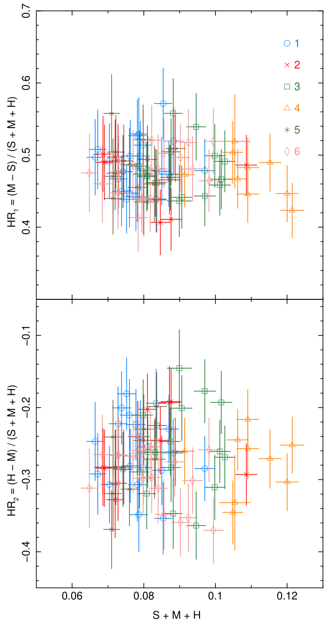
Figure 2. Hardness ratios HR_1 = (M - S)/(S + M + H) (upper panel), and HR_2 = (H - M)/(S + M + H) (lower panel) plotted against the light curve of all the energy bands ( S + M + H ).
