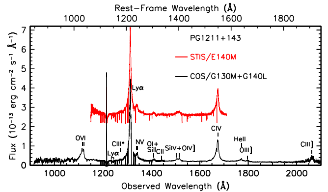
Figure 1. Merged HST /COS G130M and G140L spectra of PG 1211+143 (black) compared to the 2002 STIS/E140M spectrum (red). Wavelengths on the lower horizontal axis and fluxes are observed units. The upper horizontal axis shows wavelengths in the rest frame of PG 1211+143 at z = 0.0809 . For clarity, the STIS spectrum has been offset vertically by 2.2 \times 10^{-13} \text{ erg cm}^{-2} \text{ s}^{-1} \text{ \AA}^{-1} . Prominent emission lines are marked. An earth symbol denotes the strong geocoronal \text{Ly}\alpha emission line. All narrow absorption features are either foreground ISM or IGM absorption lines. The broad \text{Ly}\alpha absorption feature in the COS spectrum is marked above the spectrum in the blue wing of the \text{Ly}\alpha emission line.
