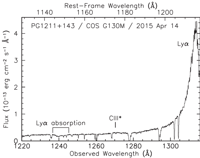
Figure 2. HST /COS G130M spectrum covering wavelengths in the blue wing of the Ly \alpha emission line of PG 1211+143. The lower horizontal axis is the observed wavelength in angstroms. The upper horizontal axis gives wavelengths in the rest frame of PG 1211+143 at z = 0.0809 . The broad feature labeled “Ly \alpha absorption” at an observed wavelength of 1240 Å is weak or absent in archival spectra. Emission lines of C III* \lambda 1176 and Ly \alpha in PG 1211+143 are labeled. All other narrow absorption lines arise in foreground interstellar or intergalactic gas.
