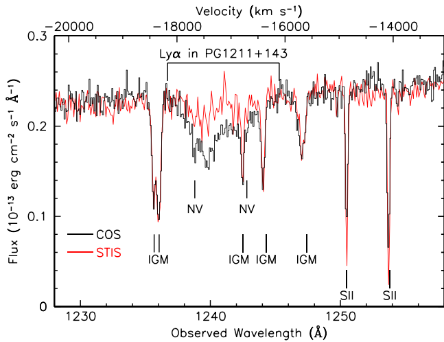
Figure 4. Comparison of the STIS E140M spectrum of PG 1211+143 to the HST /COS G130M spectrum in the region around the broad Ly \alpha absorption feature shows that the absorption feature has varied. The red line is the STIS data binned by 6 pixels; the black histogram is the COS spectrum binned by 8 pixels. The lower horizontal axis is the observed wavelength in ångströms. The upper horizontal axis gives the outflow velocity of Ly \alpha in the rest frame of PG 1211+143 at z = 0.0809 . Interstellar and intergalactic lines are labeled as in Figure 3.
